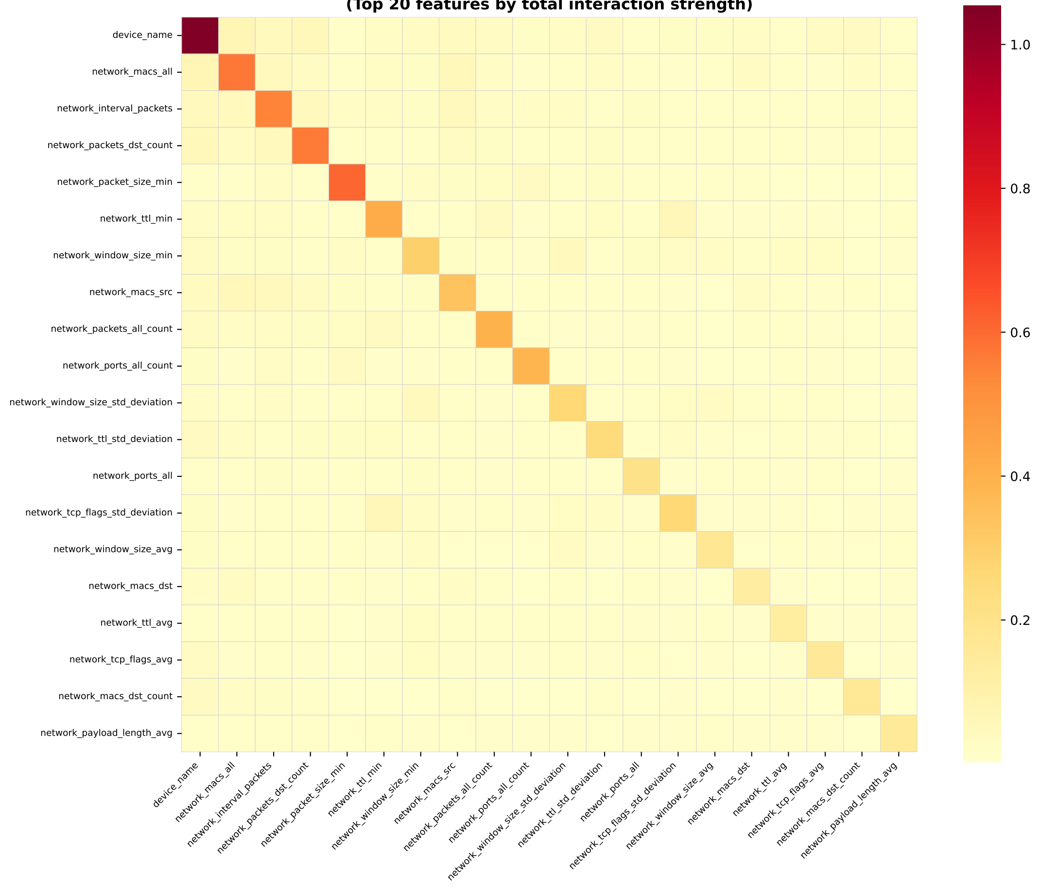
SHAP Interaction Values — XGB on CIC_IIoT_2025 (Top 20 features by total interaction strength)
